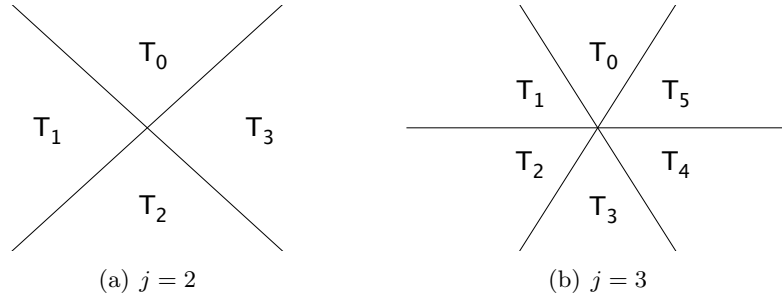
Figure 3.1: the families \{T_k / k = 0, \dots, 2j - 1\} for j = 2, 3
